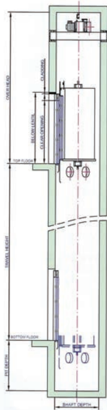
LIFT WELL ELEVATION
